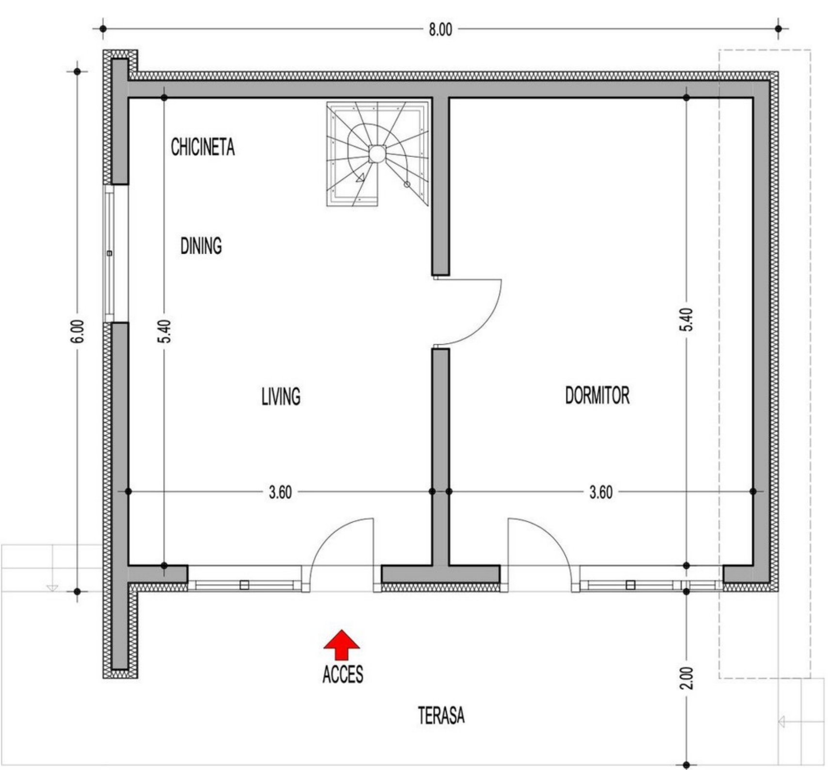
Chalet Retreat - Plan parter
