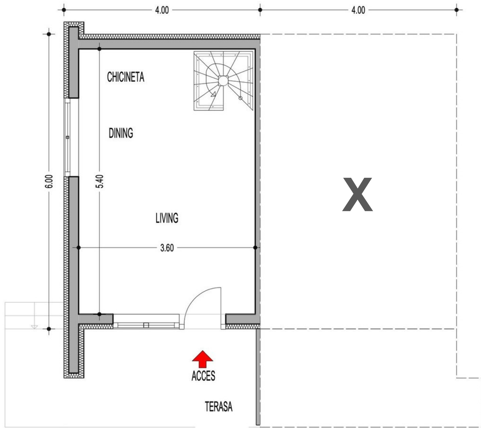
Loft Escape- Plan parter
